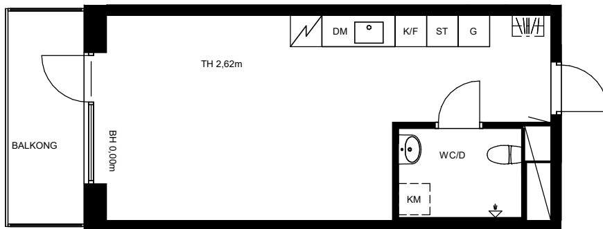
Plan 2
