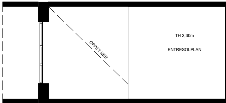
Plan 5, entresol
