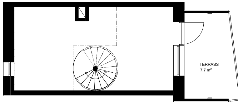
Plan 2
